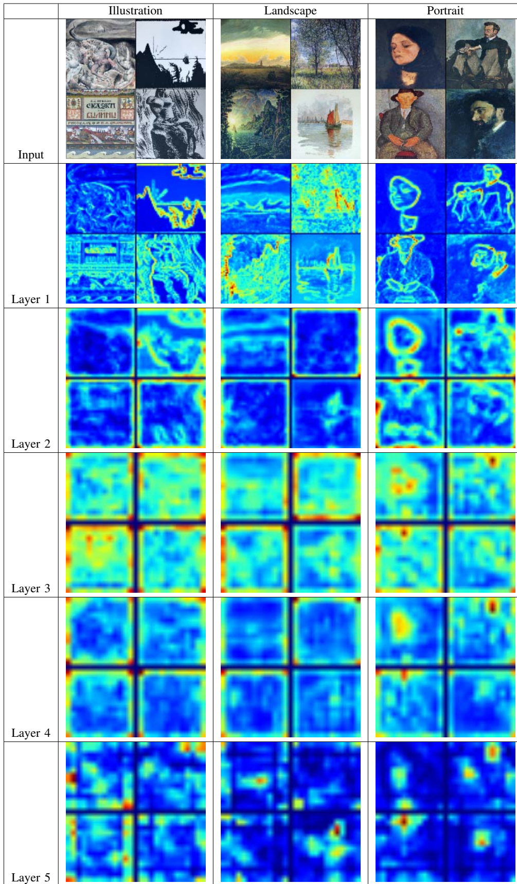
Fig. 3: The complete visualization (conv1-5) of neurons' responses in the genre classification.
